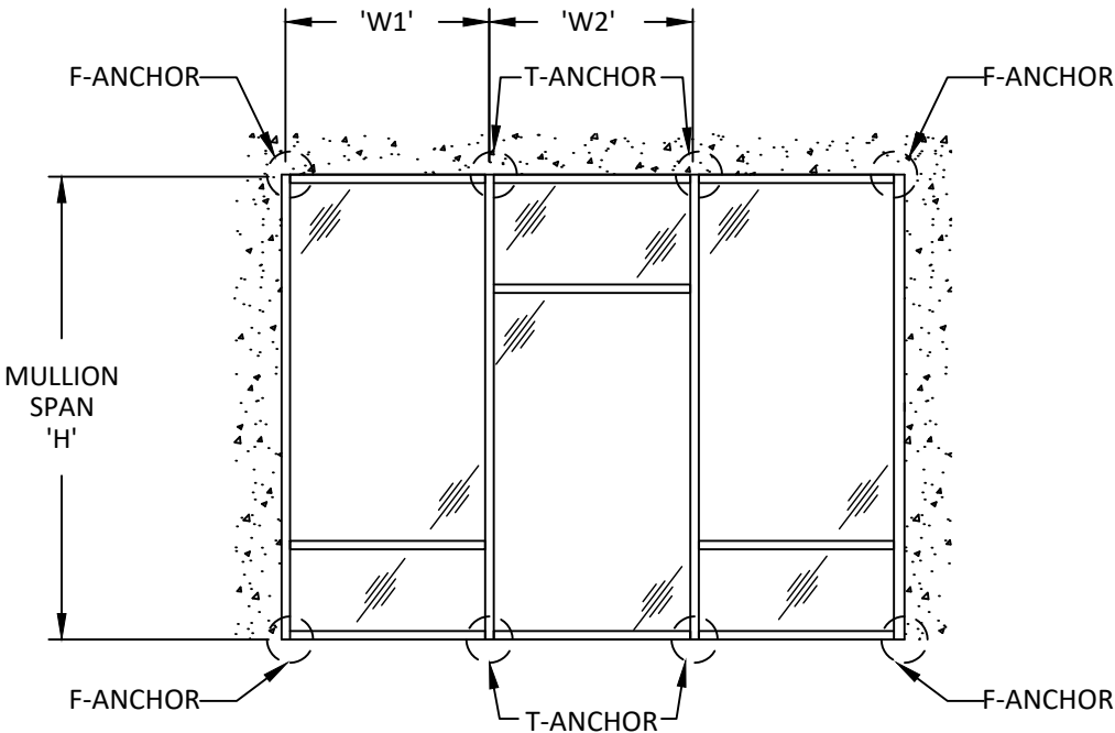
SINGLE SPAN ANCHOR LAYOUT
