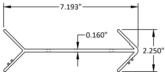
5 1/4" CORNER ANCHOR SLEEVE E9-7093
