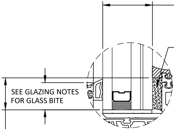
GLAZING OPTION A MAY BE USED WITH INSIDE & OUTSIDE CORNERS
