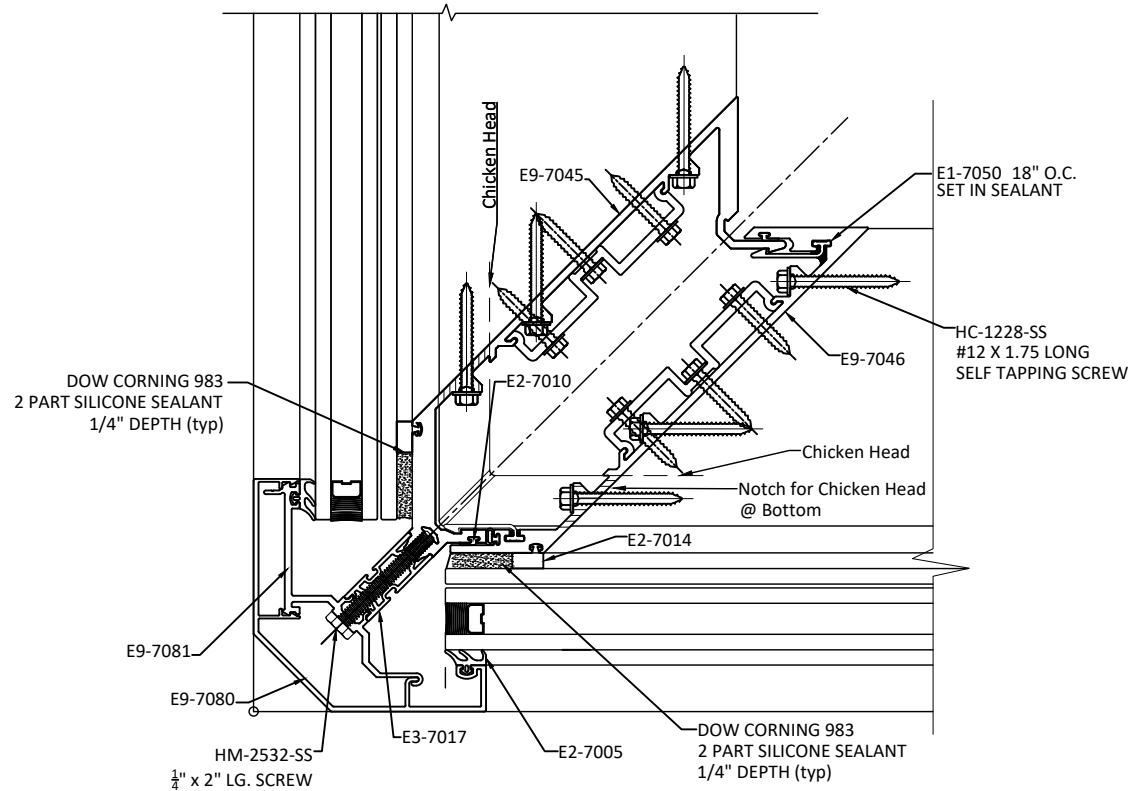
Q 8 HORIZONTAL SECTION OUTSIDE CORNER SINGLE & MULTI SPAN
