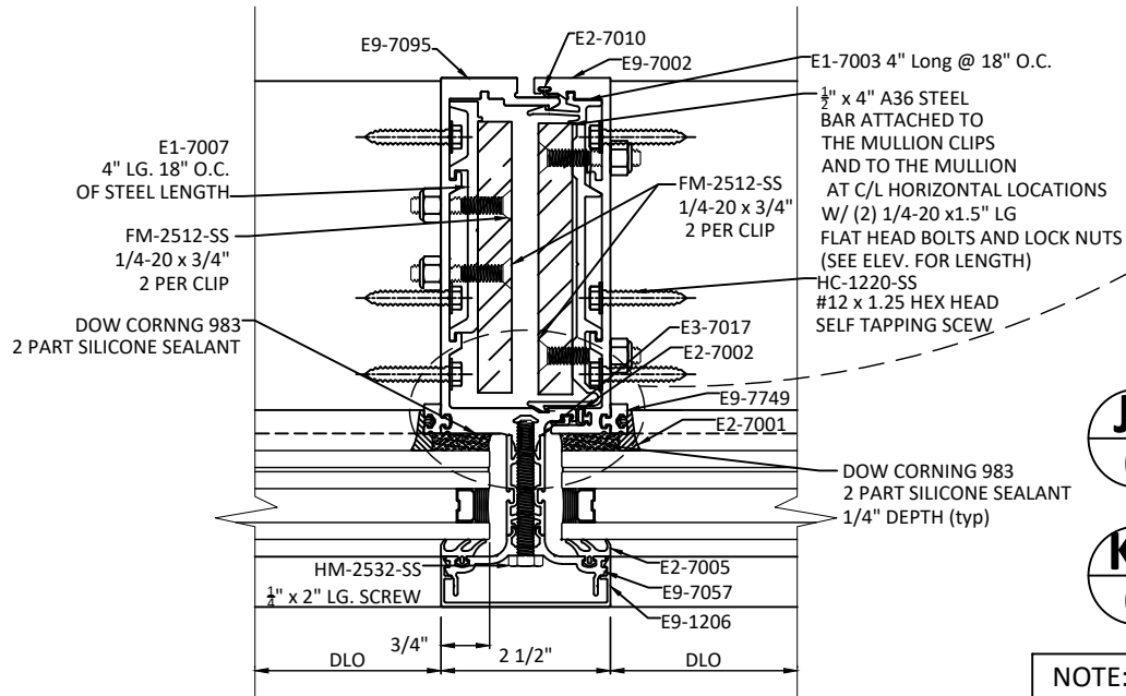
J1 HORIZONTAL SECTION 6 INT. REINF. VERTICAL - W/ ADAPTOR PRESSURE PLATE (CAPTURED)
