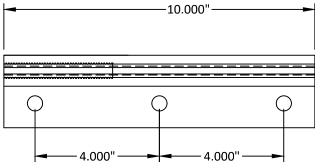
LH MULLION ANCHOR E1-7015 (E1-7014 MIRRORED)
