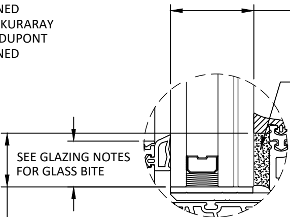
GLAZING OPTION B NOT FOR USE WITH INSIDE & OUTSIDE CORNERS
