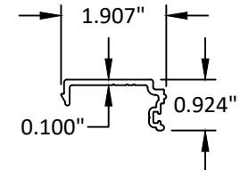
GLAZING FILLER E2-7018
