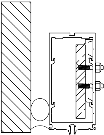
REINFORCED JAMB
