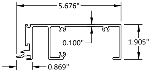
5 1/4" SSG SILL/HORIZONTAL E9-7023
