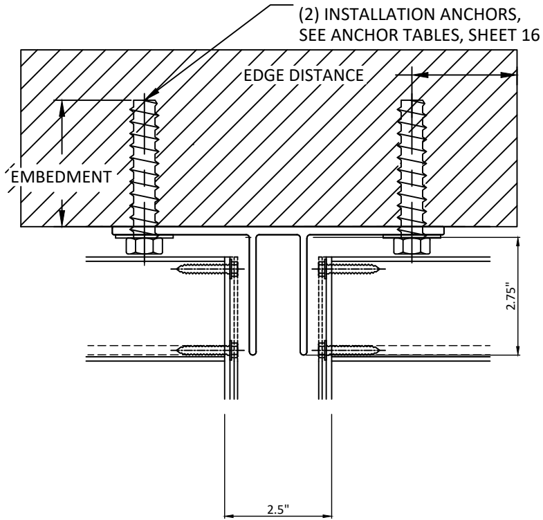
V1 14 FRONT VIEW T-CLIP AT VERTICAL MULLION HEAD
