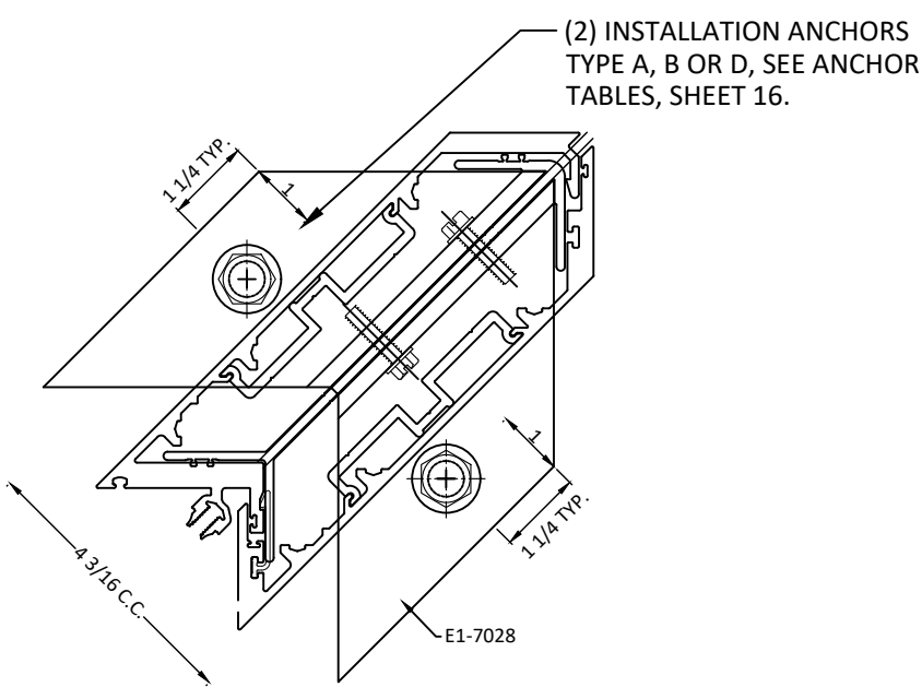
INSIDE 90 DEGREE ANCHORS INTO CONCRETE SUBSTRATES
