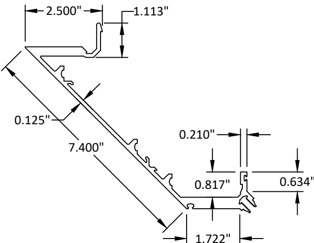
5 1/4" OUTSIDE CORNER MALE MULLION E9-7045
