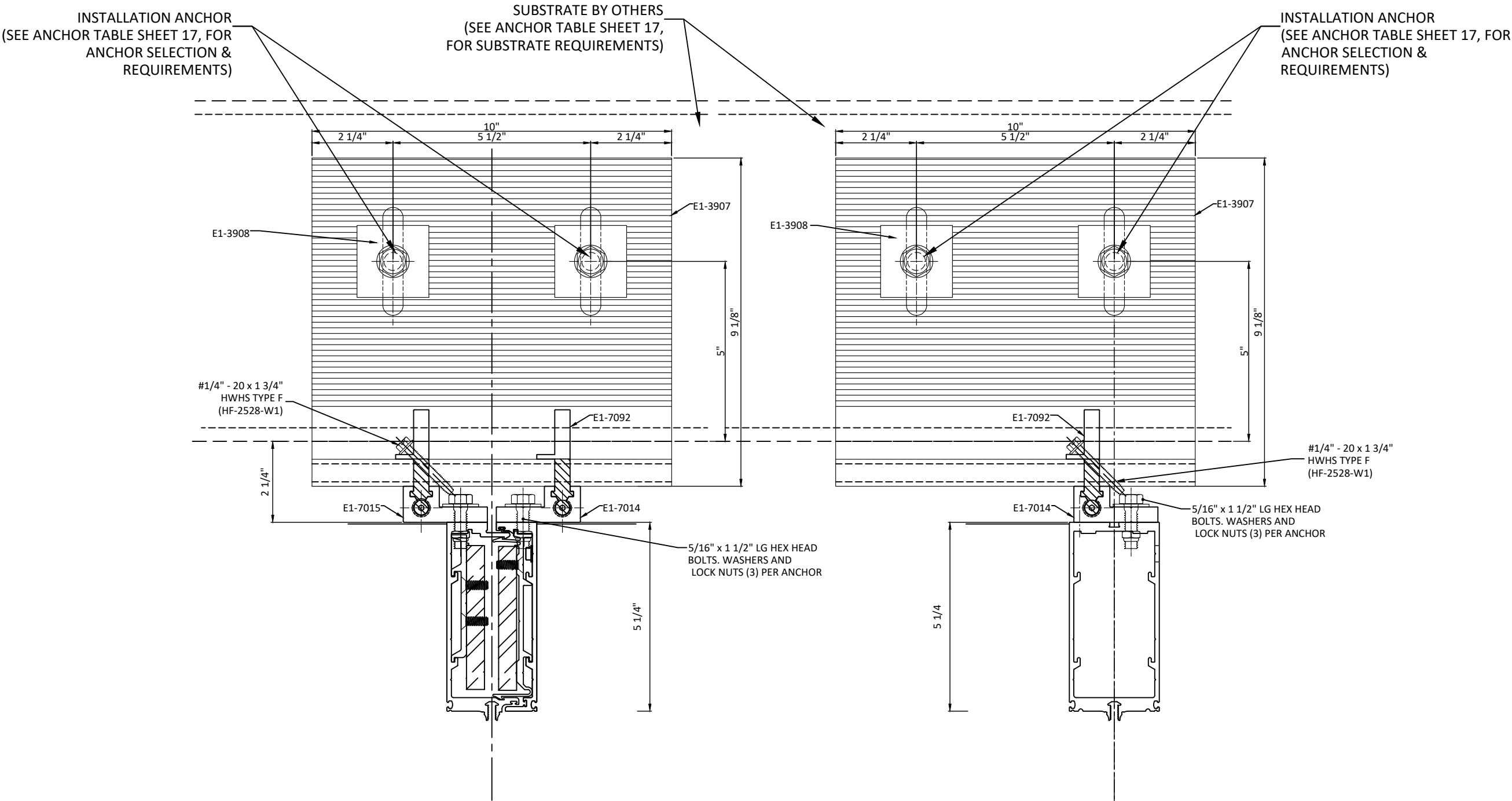
X 18 HORIZONTAL SECTION DEAD LOAD L-ANCHOR INTERMEDIATE VERTICAL MULLION
