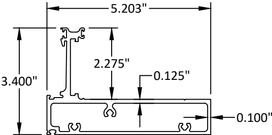
5 1/4" HEAD/HORIZONTAL E9-7027
