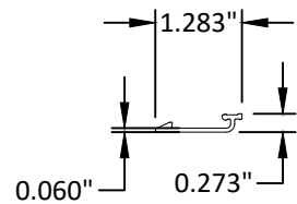
CORNER ANTI-BUCKLING CLIP E9-7050
