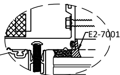
L1 HORIZONTAL SECTION 6 REINF. JAMB - E.T.A. WITHOUT ADAPTOR
