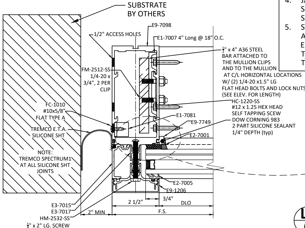
L1 HORIZONTAL SECTION 6 REINF. JAMB - E.T.A. W/ ADAPTOR - MULTI-SPAN
