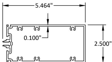
5 1/4" INTERMEDIATE HORIZONTAL E9-7097
