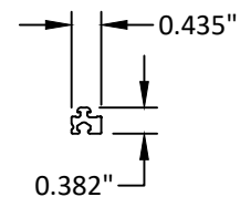
1/4" ADAPTOR E9-7749
