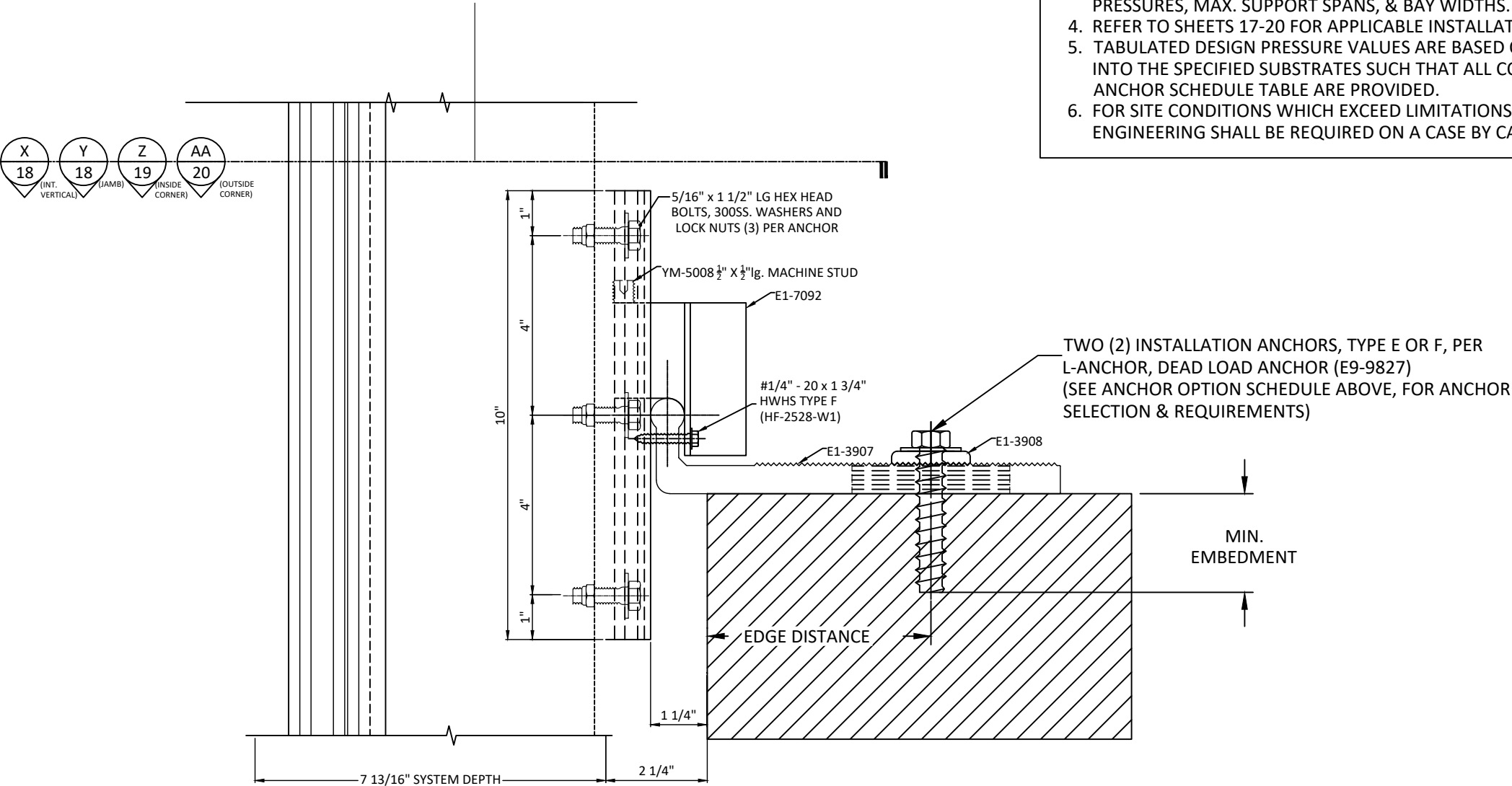
W 17 VERTICAL SECTION DEAD LOAD L-ANCHOR TYP.
