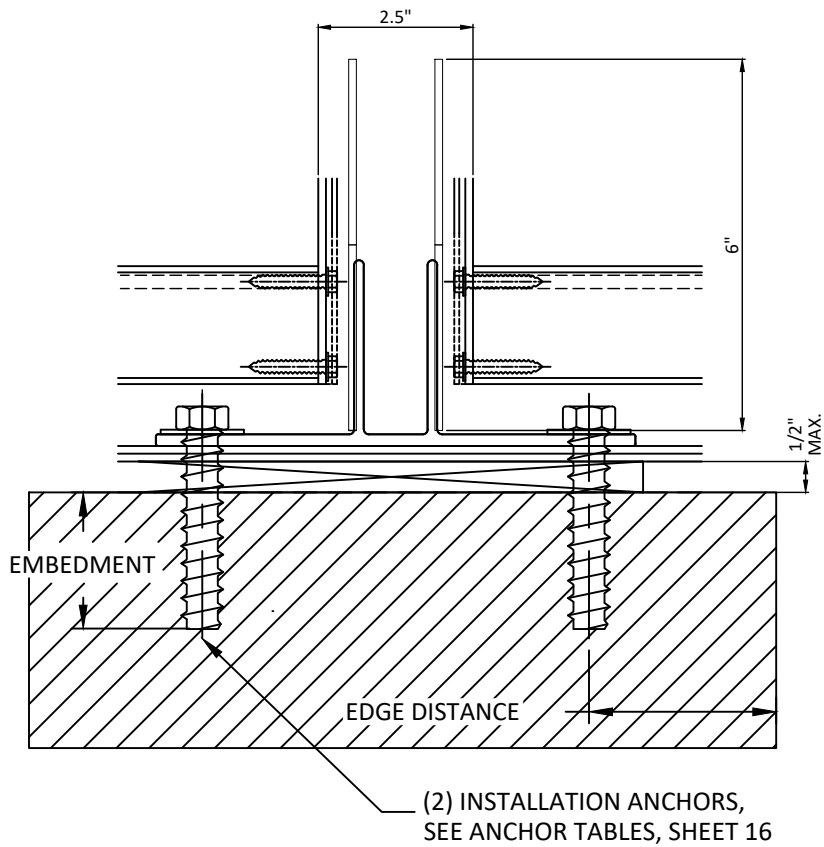
U 14 FRONT VIEW T-CLIP AT VERTICAL MULLION WITH SILL STARTER
