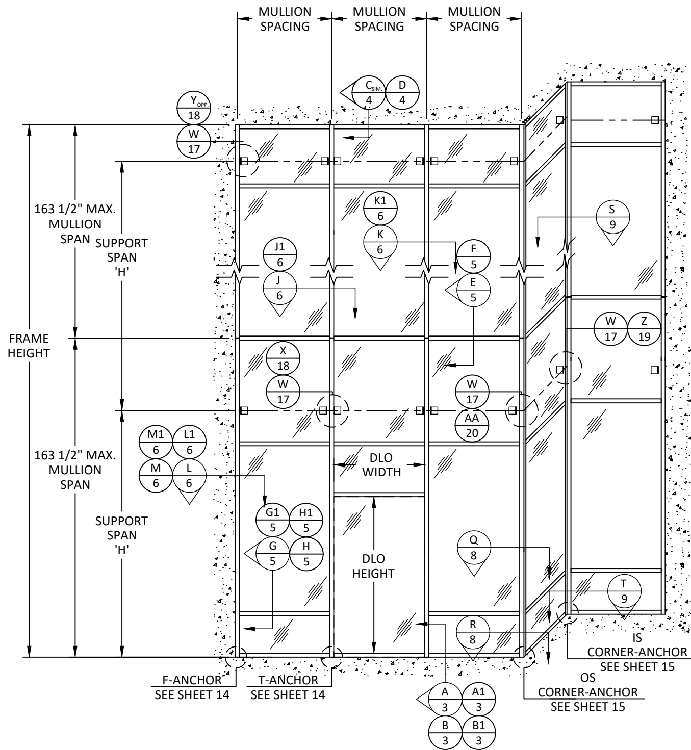
ELEVATION MULTI-SPAN
