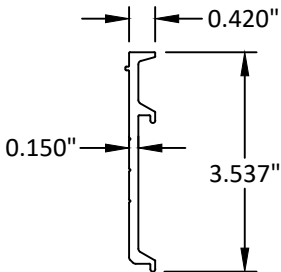
5 1/4" MULLION REINFORCEMENT CLIP E1-7007
