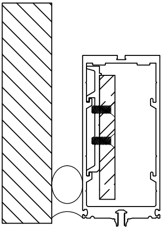
REINFORCED JAMB
