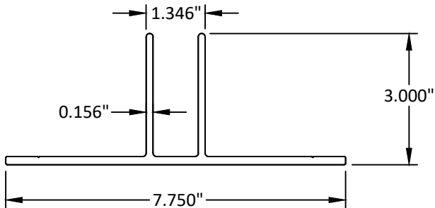
MULLION T-ANCHOR (WINDOW WALL) E1-7024
