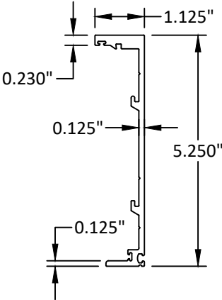
5 1/4" FEMALE MULLION HALF E9-7002
