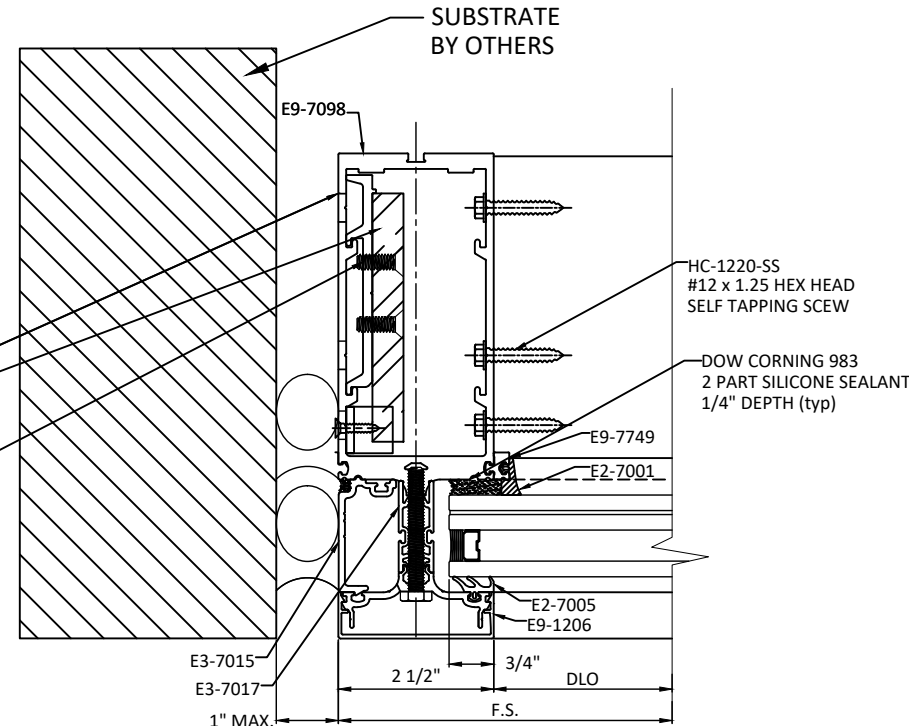
M1 HORIZONTAL SECTION 6 REINF. JAMB - BACKER ROD & SEALANT W/ ADAPTOR - SINGLE-SPAN
