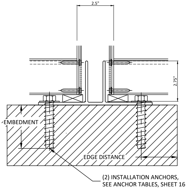
V 14 FRONT VIEW T-CLIP AT VERTICAL MULLION WITHOUT SILL STARTER
