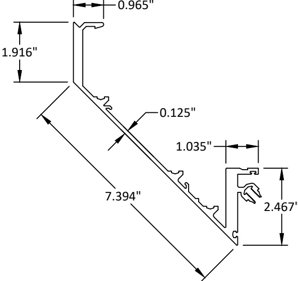
5 1/4" INSIDE CORNER MALE MULLION E9-7047
