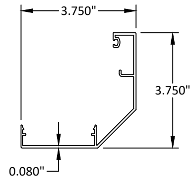
90 DEG. OUTSIDE CORNER FACE COVER (1 5/16" GLASS) E9-7080
