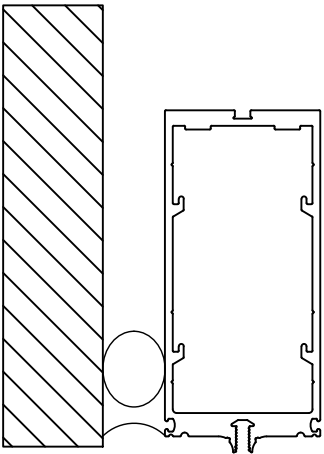
UNREINFORCED JAMB
