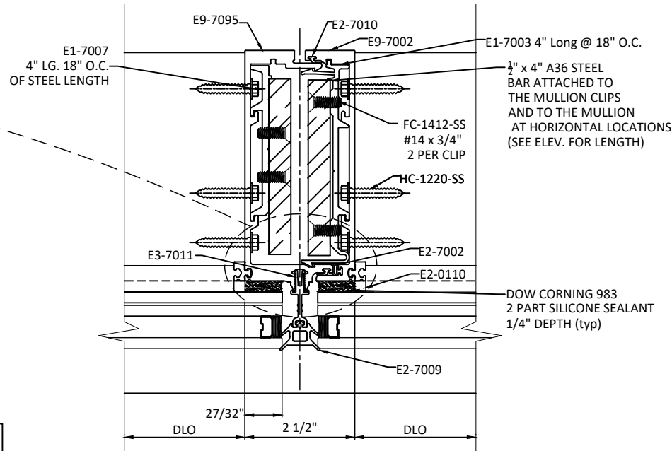
K1 HORIZONTAL SECTION 6 INT. REINF. VERTICAL - W/ ADAPTOR SSG
