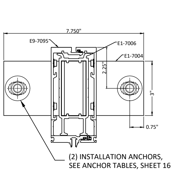
T-CLIP ANCHORS AT MULLIONS W/ SILL STARTER
