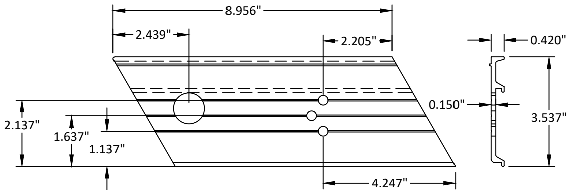
5 1/4" LH MULLION SLEEVE E1-7022 (E1-7021 MIRRORED)
