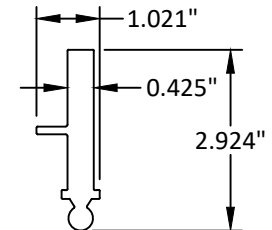
BRACKET SLEEVE E9-7092
