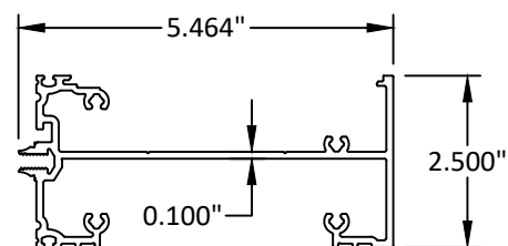
5 1/4" OPEN BACK HEAD/SILL E9-7099
