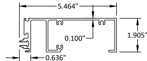
5 1/4" SILL/HORIZONTAL E9-7096
