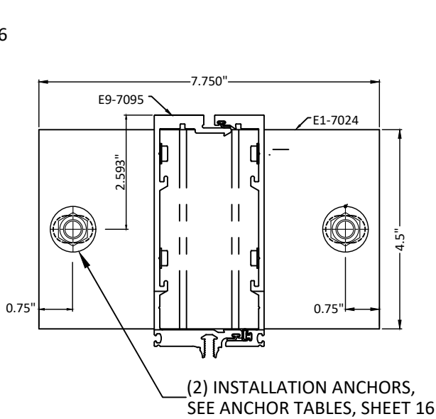
T-CLIP ANCHORS AT MULLIONS W/ OUT SILL STARTER
