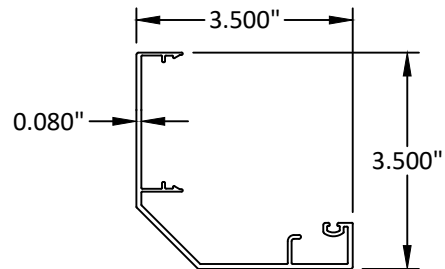
90 DEG. OUTSIDE CORNER COVER E9-7056
